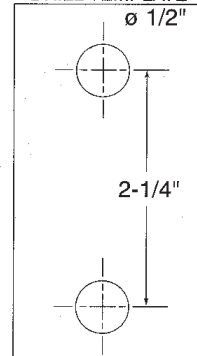
DRILL TEMPLATE
